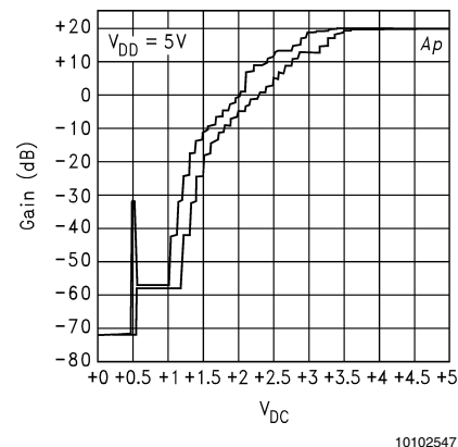
FIGURE 2. Typical part-to-part gain variation as a function of DC-Vol control voltage
